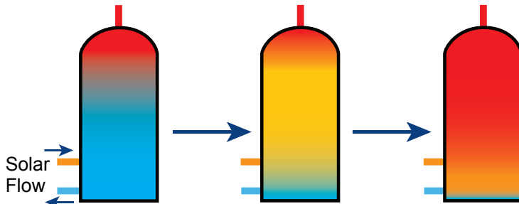
Fig 1. Solar Heating
