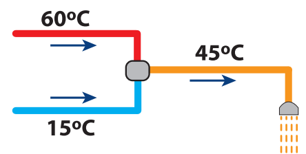
Fig 3. Temperature Mixing
