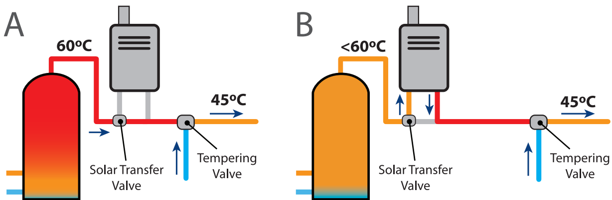
Fig 5. Gas Boosting
